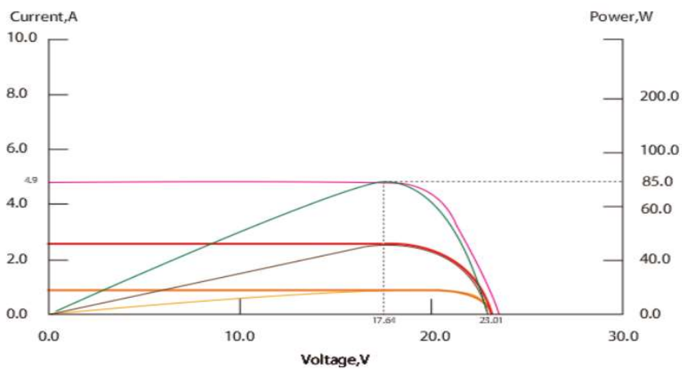
Current-Voltage & Power-Voltage characteristics various irradiance levels
